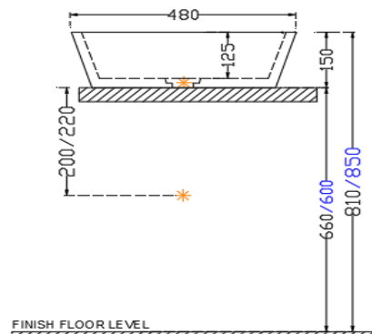
INSTALLATION SIDE VIEW
