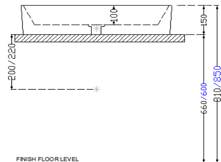
INSTALLATION SIDE VIEW
